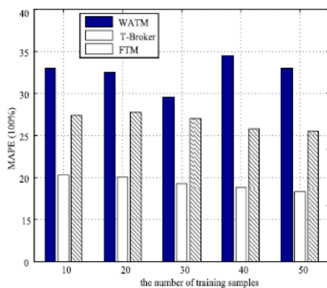
Fig 7: The values of MAPE with a small number of training samples.
