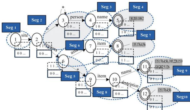
Fig 3: divide the global automaton with granularity
