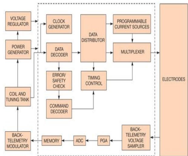
Fig5: A Receiver and a Simulator In An Internal Unit Act As The Engine Of A Cochlear Implant
