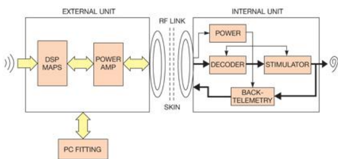
Fig4: a system monitors critical electrical and neural activities in the implants and transmits the activities back to the external unit
