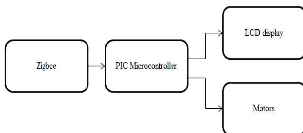
Fig 1.2 Block Diagram of Receiver Section
