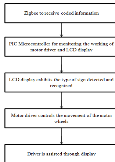
Fig 11. Flowchart of Receiver section
