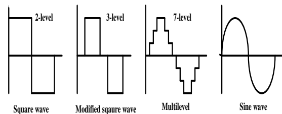
Fig- 1: Inverter output waveforms
