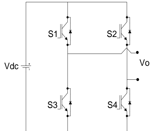
Fig-6: A 3-Level Cascaded H-Bridge Inverter
