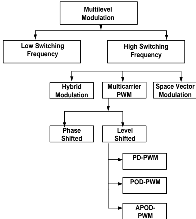
Fig-7: Classification of multilevel modulation methods
