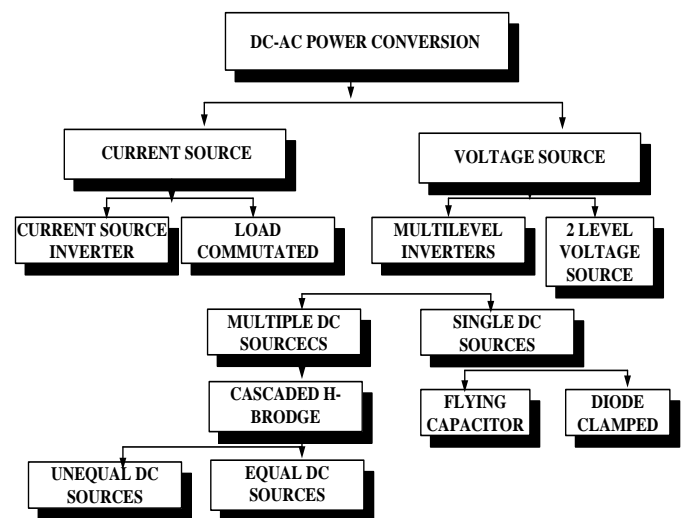
Fig-2: Classification of Multilevel converter
