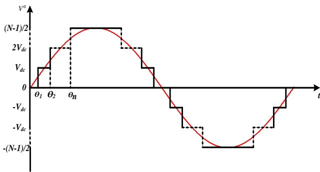
Fig-3.: Generalized stepped waveform of multilevel inverters
