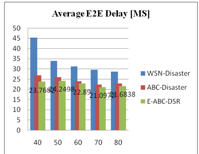
Fig -3: Average E2E Delay
