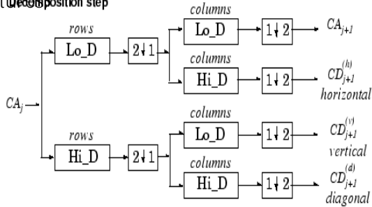
Figure 2- Two level DWT of original image.
