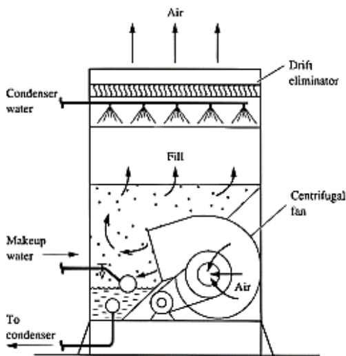
Fig-12: Counter flow forced draft.
