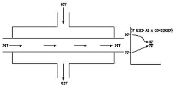
Fig -2: Cross flow type heat exchanger.
