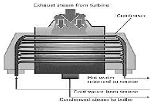
(a) Water cooled condenser
