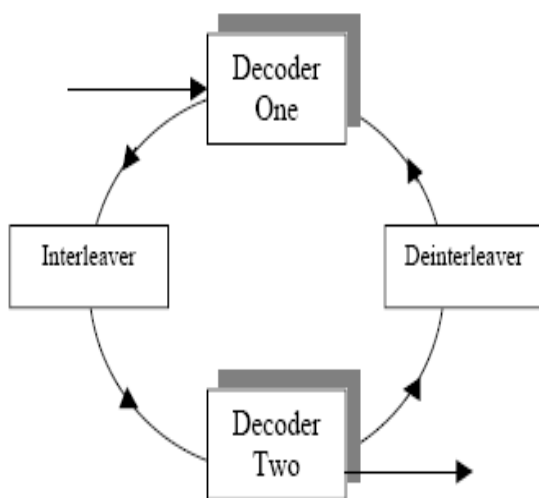
Fig.2 Turbo decoder
