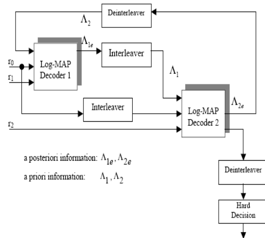
Fig. 3 Log-MAP algorithm
