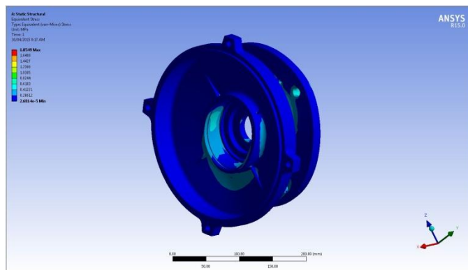
Figure 6: Stress distribution
