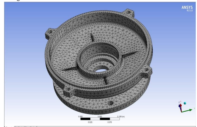
Figure 5: FEA Model
