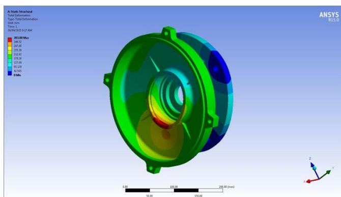
Figure 8: Deformation change.
