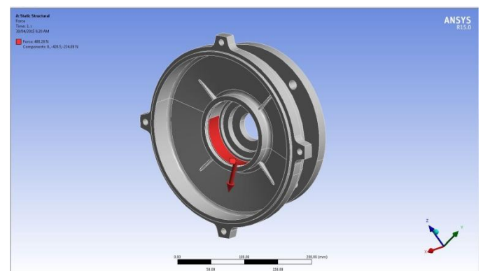
Figure 6: Load application
