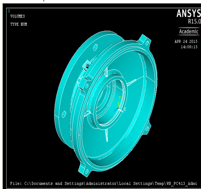
Figure 4: CATIA model flange of B5 imported in ANSYS
