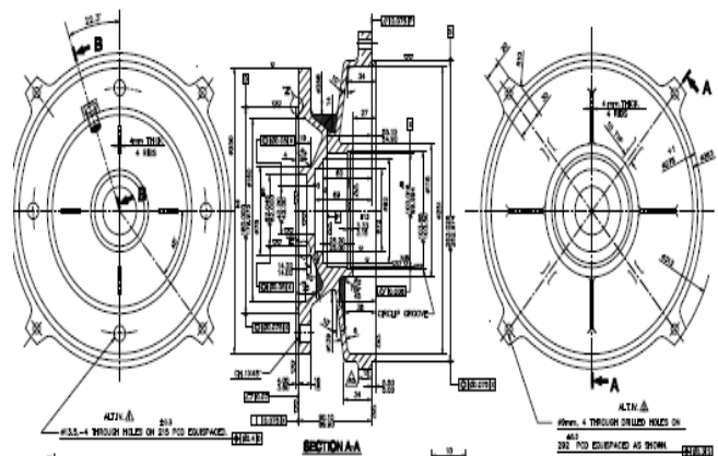
Figure 2: Actual dimensions of flange of B5 type motor
