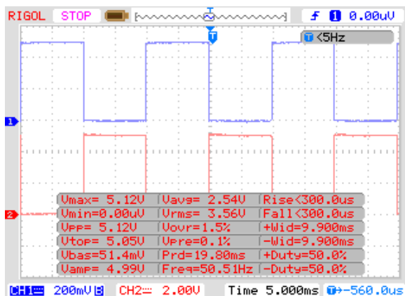
Fig 8: Switching Waveforms of inverter: Switching Frequency: 50Hz
