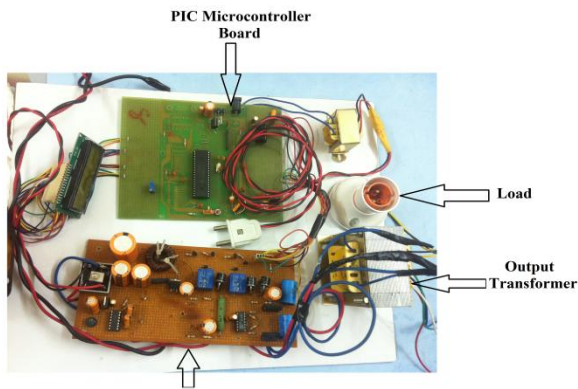
Fig 6: Hardware Set-up
