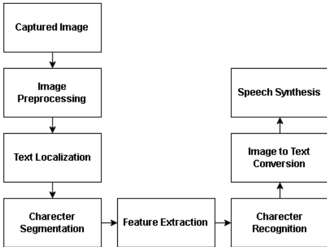
Fig 4. Working Principle
