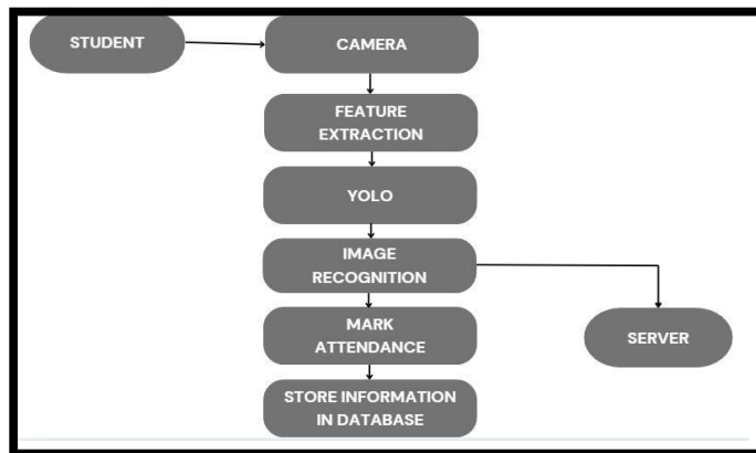
Fig -2: Working of the Model
