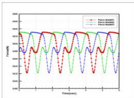
Fig.8 Forces on each blade as it rotates, and the force variations on each blade is obviously affected by the floating body and the struts.
