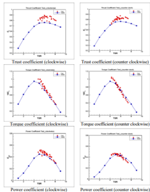
Fig.10 Comparison of the measured data and the RANS computational results
