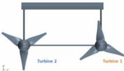
Fig.11 The relative position between turbine 1 and turbine 2. The perspective is downstream of the NKT turbine.
