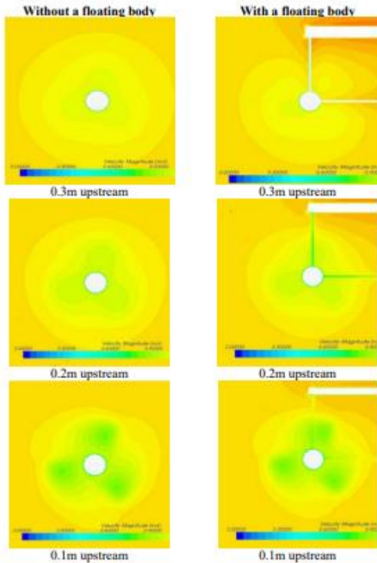
Fig. 7 The flow field at different locations upstream of turbine blades with and without a floating body
