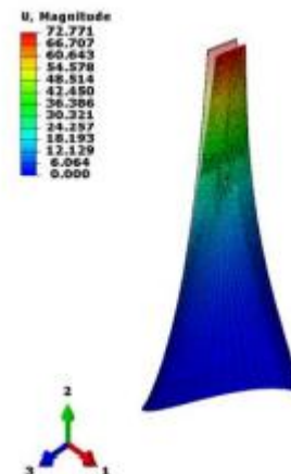
Fig. 16 The deformation at the tip of the blade is 72.77mm, which is about 3.83% relative to the blade length.
