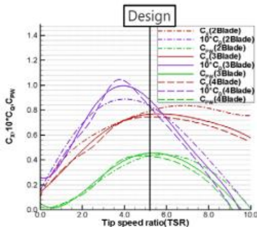
Fig. 5 Computational results of the analysis of the three different blade numbers, and the position marked by the black line is the design point.
