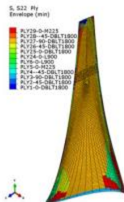
Fig. 15 The stress distribution of the 27 th layer fibre (DBLT1800 90°).
