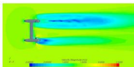
Fig. 12 The flow filed of one side malfunction situation
