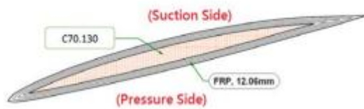
Fig. 14 The FRP sandwich structure, and blade is divided into suction side and pressure side.
